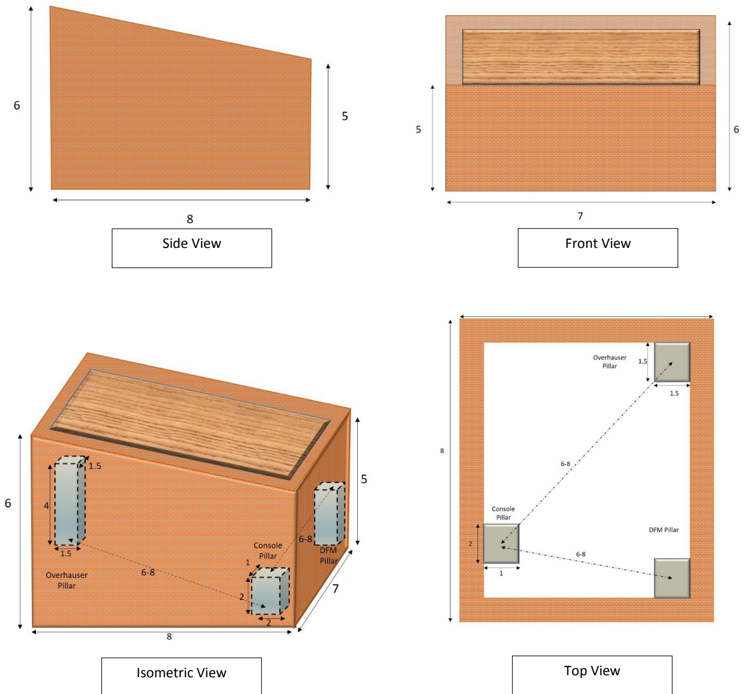
Fig. 2 Schematic diagram of geomagnetic chamber
